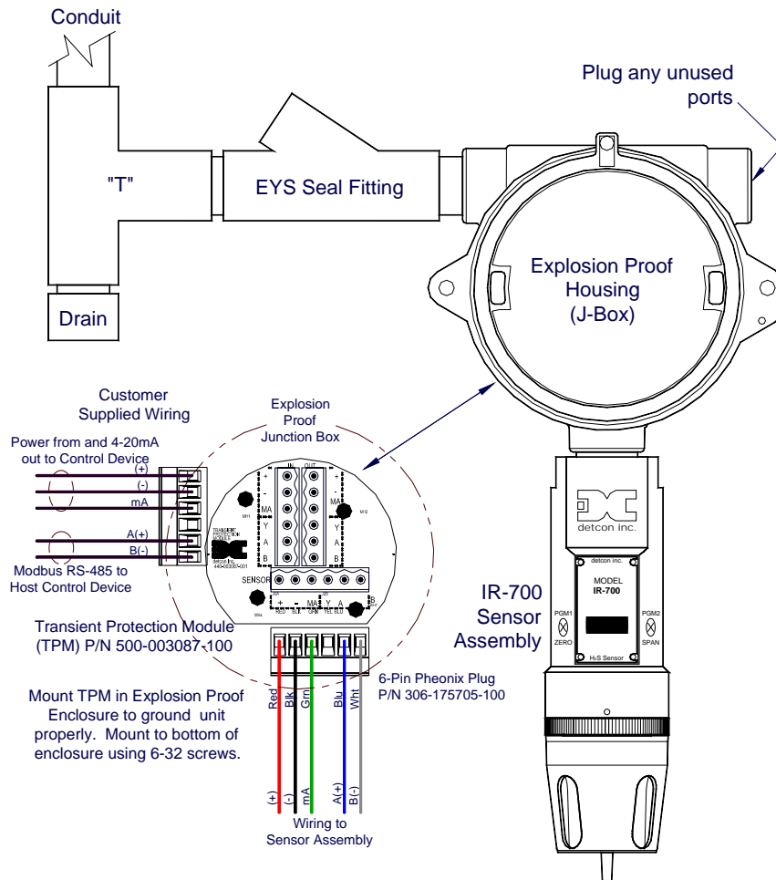
Figure 10 Typical Installation
