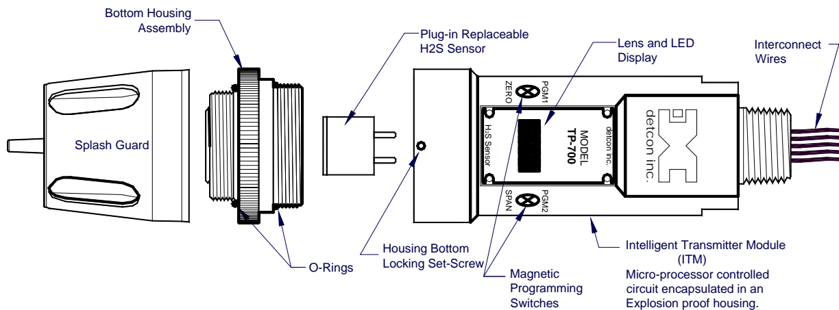
Figure 15 Sensor Assembly
