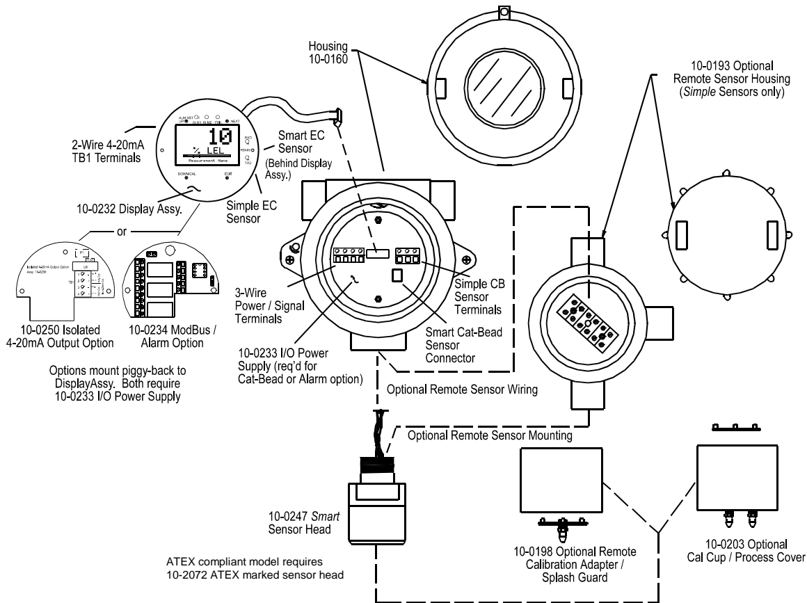
Figure 2-3: Outline Drawing
