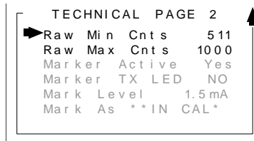
Figure 7-4: 4-20mA Input "MARKER" Menus
