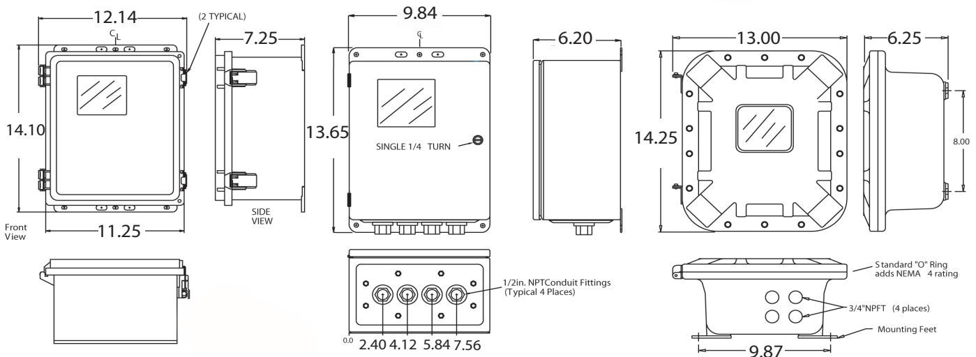
ViewSmart 200 NEMA4 Painted Steel
